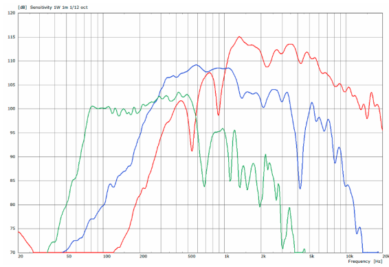
PS 1 - Frequency Response with 2-way preset
